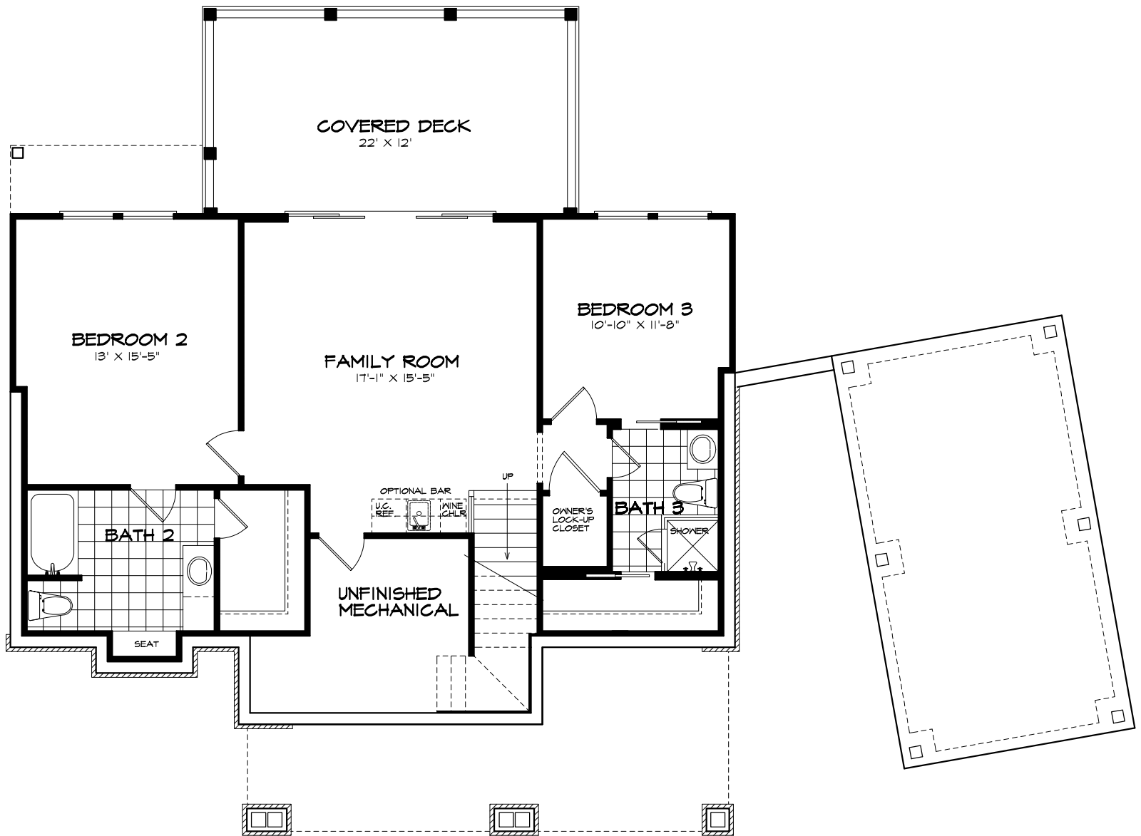
TERRACE LEVEL PLAN - 982 S.F. FINISHED AREA LAUREL "B"
