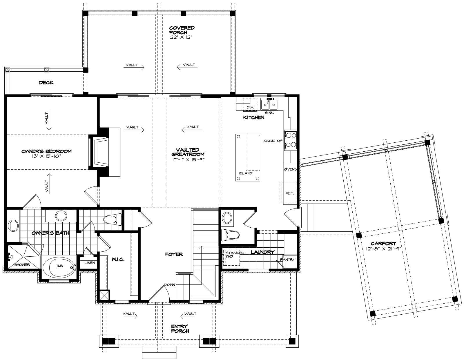
MAIN LEVEL PLAN - 1105 S.F. FINISHED AREA LAUREL "B"
