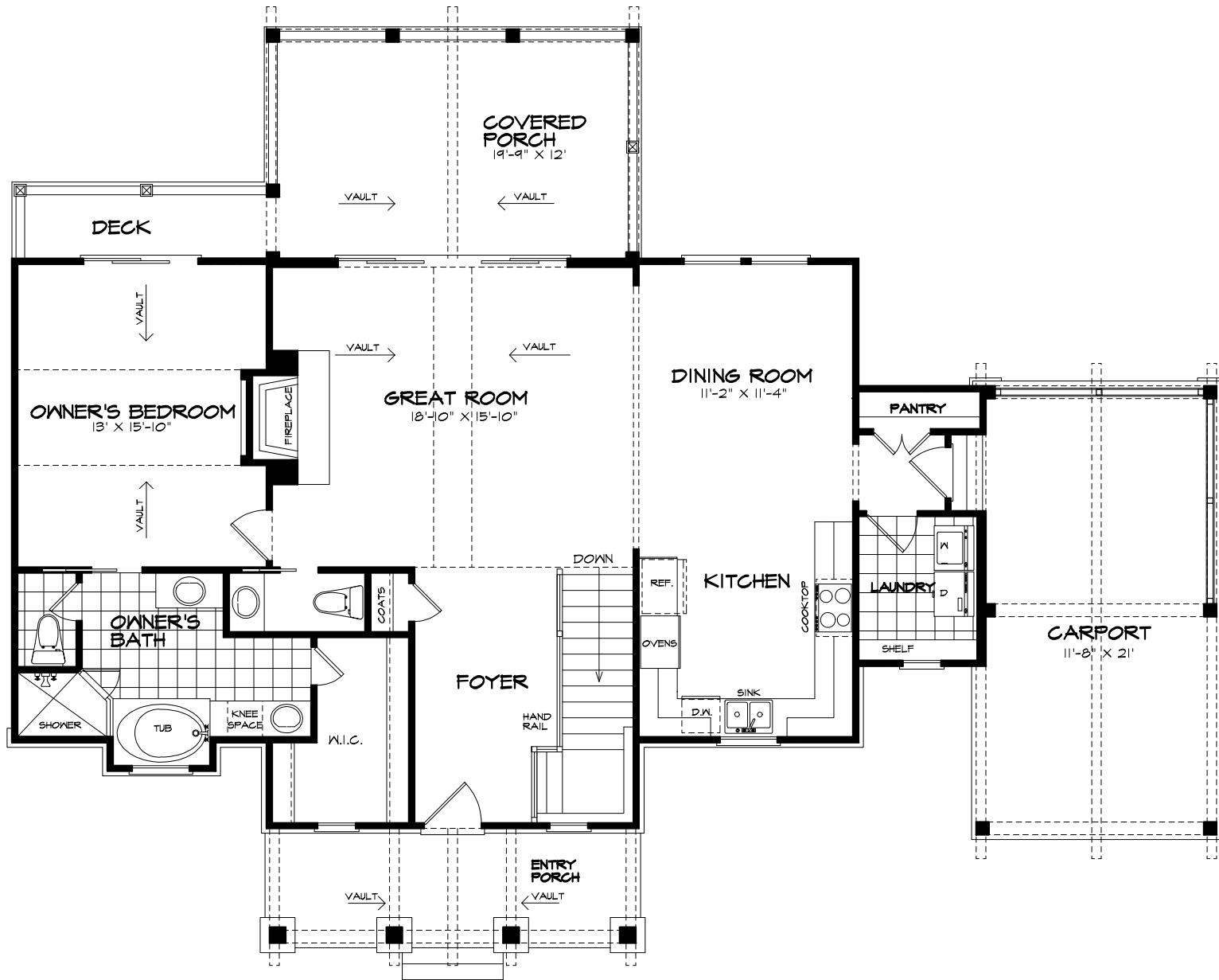
MAIN LEVEL PLAN - 1257 S.F. FINISHED AREA HICKORY "A"
